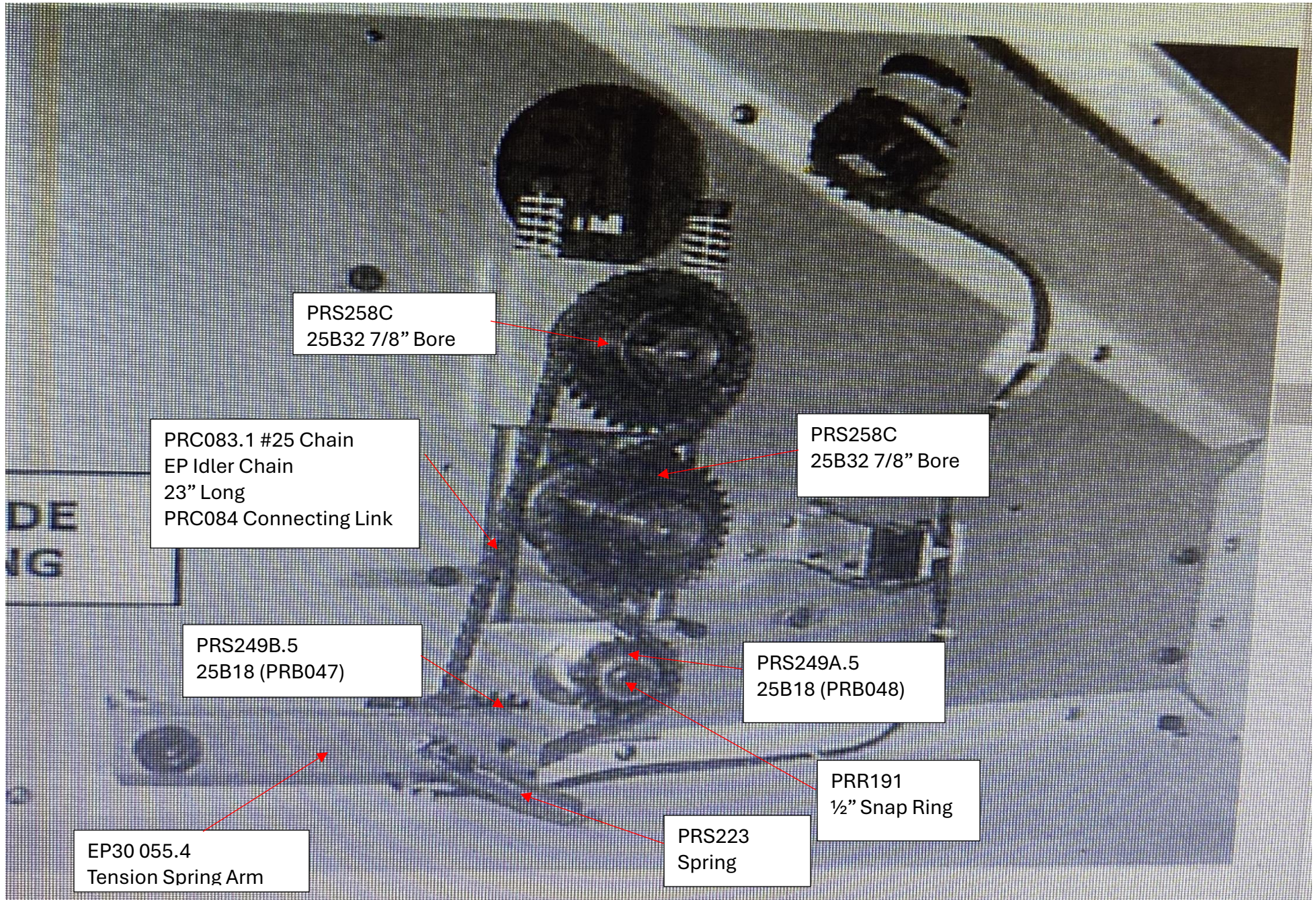
Econocraft Gears Left Side. EP30 EP44 EP60
