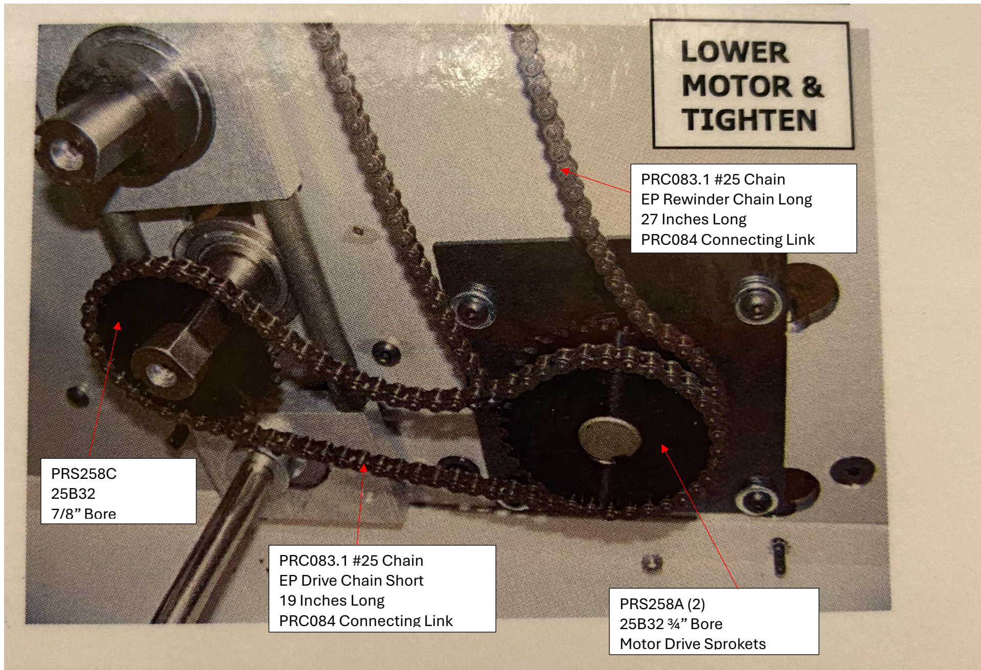
Econocraft Gears Right Side. EP30 EP44 EP60
